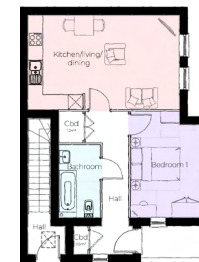
House type F Ground Floor
