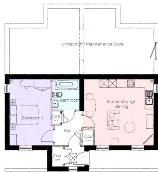
Flat type A Lower Ground Floor
