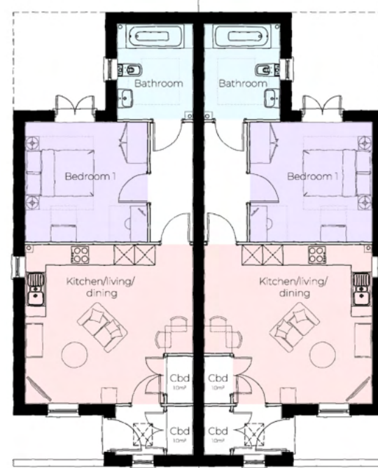
Flat type B Lower Ground Floor
